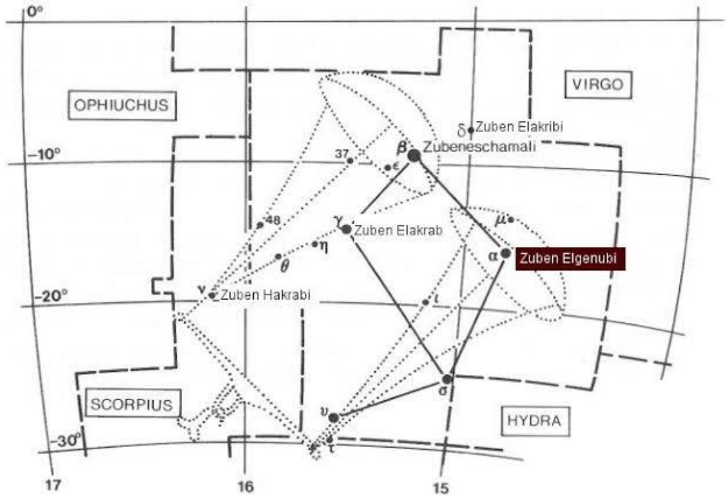
Libra. The Scales. (C26; al-Sufi, Persian, 10th Century A.D.)
